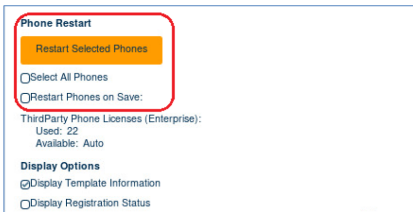
Figure 80 - Phone Restart and Display Selection Sections
