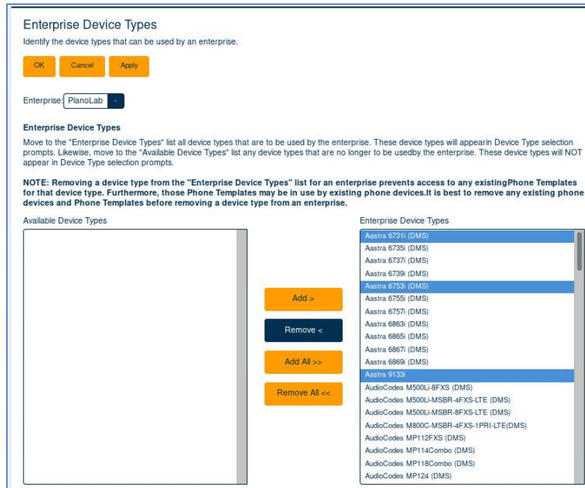
Figure 190 - Enterprise Device Types Page
