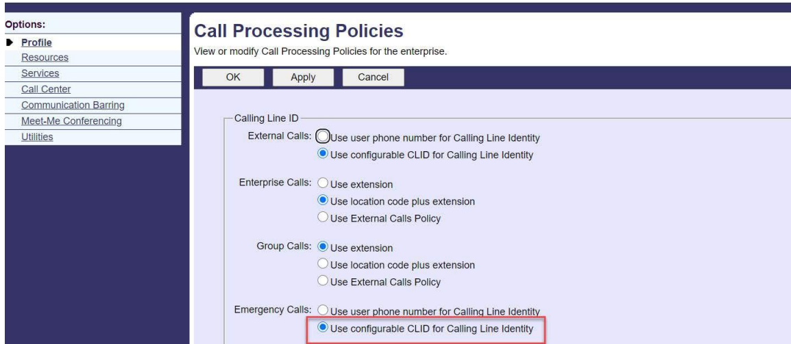
Figure 99 -Clearspan Call Processing Policies Page
