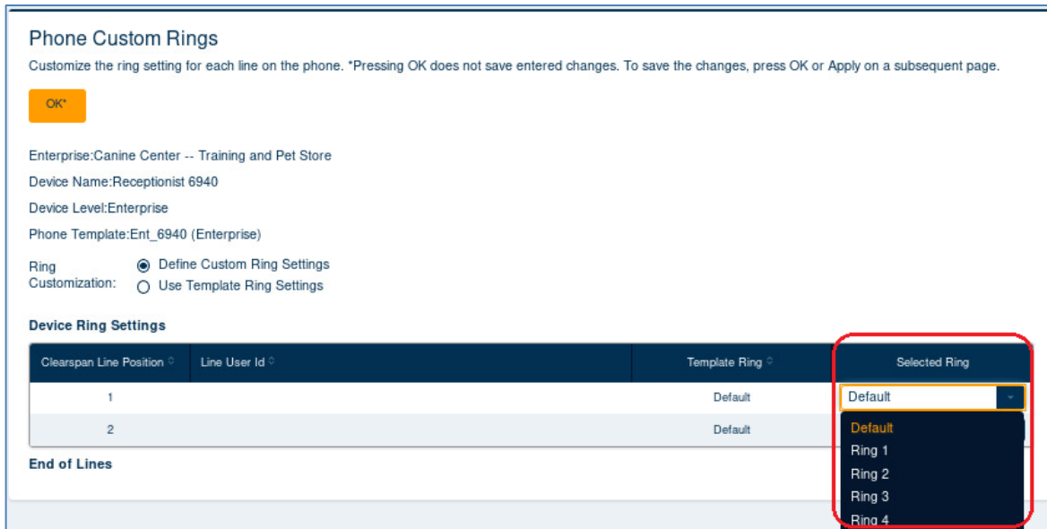
Figure 83 - Phone Custom Rings Page
