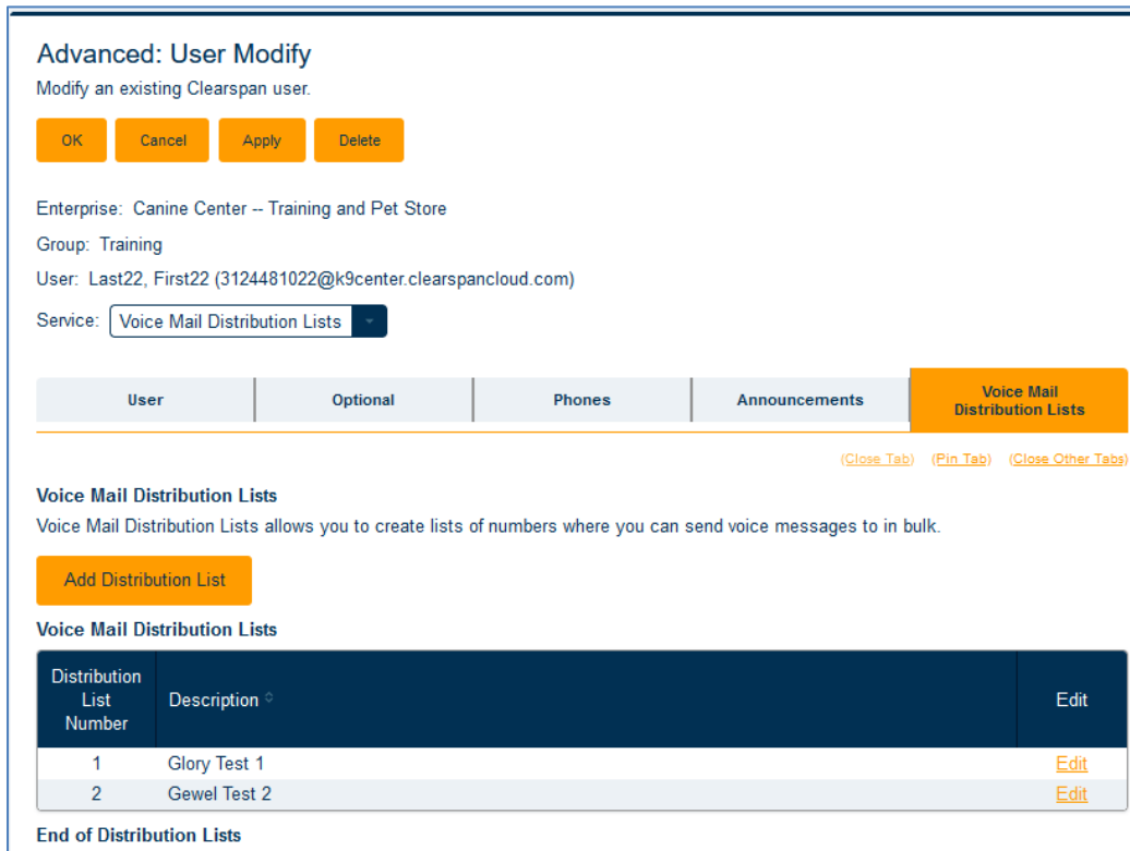
Figure 143 - Voice Mail Distribution Lists
