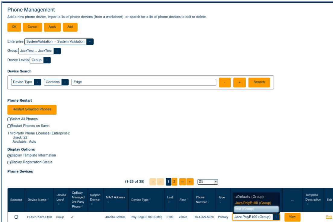
Figure 78 - Changing Template for a Phone Device
