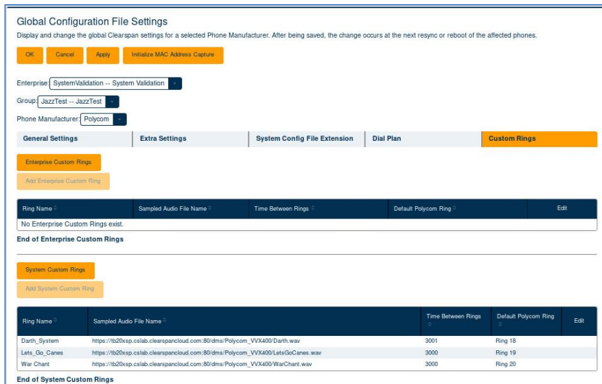
Figure 63 - Custom Rings for Polycom Phones
