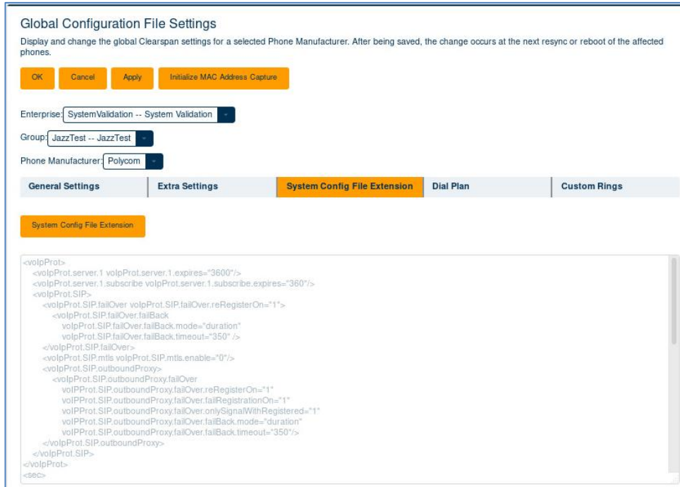
Figure 62 - System Config File Extension Settings for Polycom Phones
