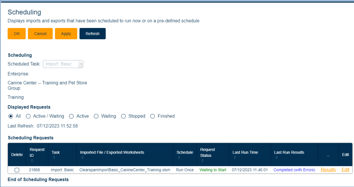
Figure 36 - Scheduling Page
