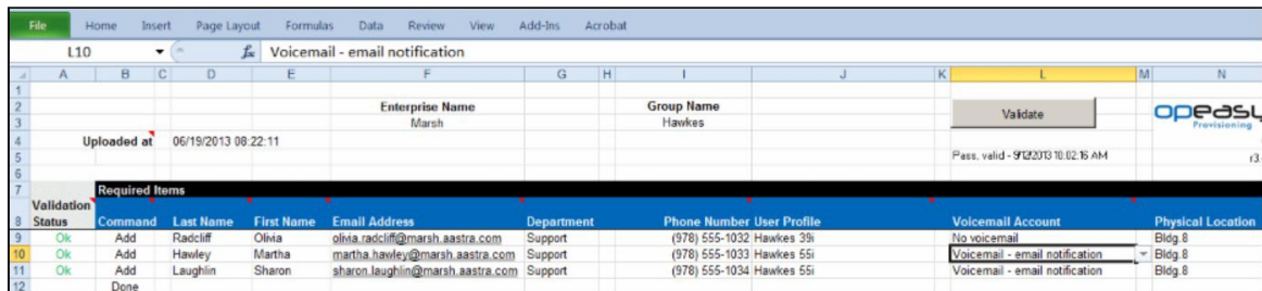
Figure 16 - Worksheet Validated
