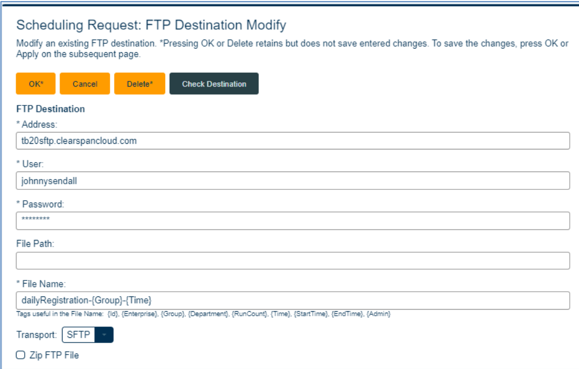
Figure 41 - Report Scheduling: FTP Destination Modify Page
